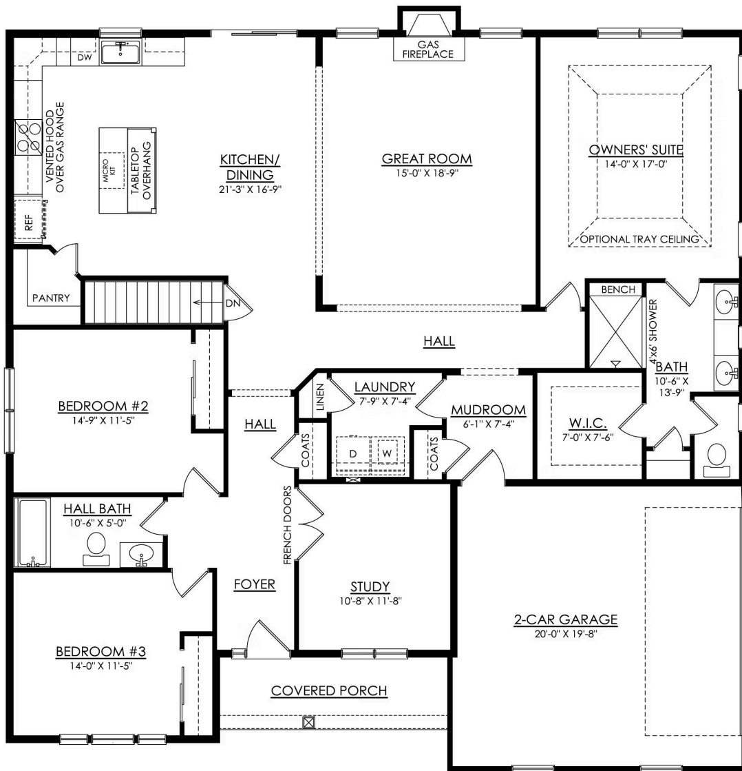
FOLINO CRAFTSMAN SE 1ST FLOOR PLAN HERITAGE
