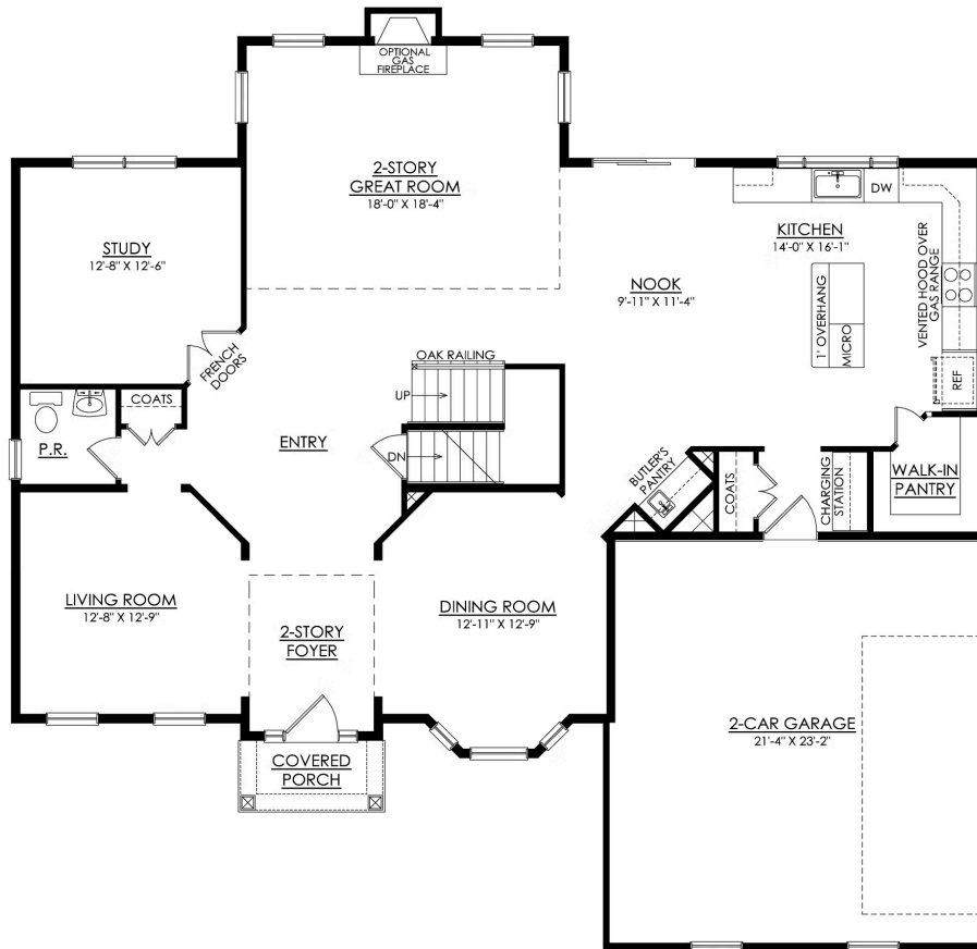
JUNIPER TRADITIONAL 1ST FLOOR PLAN HERITAGE
