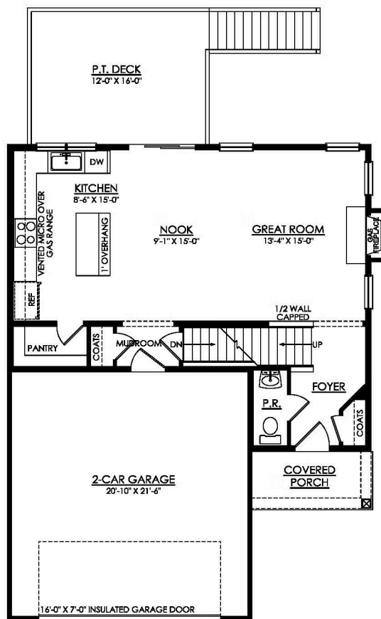
LILY 1ST FLOOR PLAN SAND SPRINGS- SS34B
