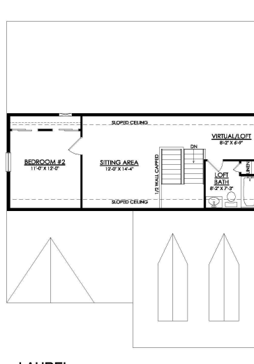
LAUREL 2ND FLOOR PLAN RE27
