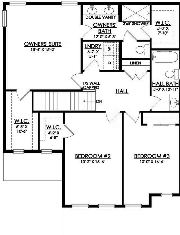
LILY 2ND FLOOR PLAN
