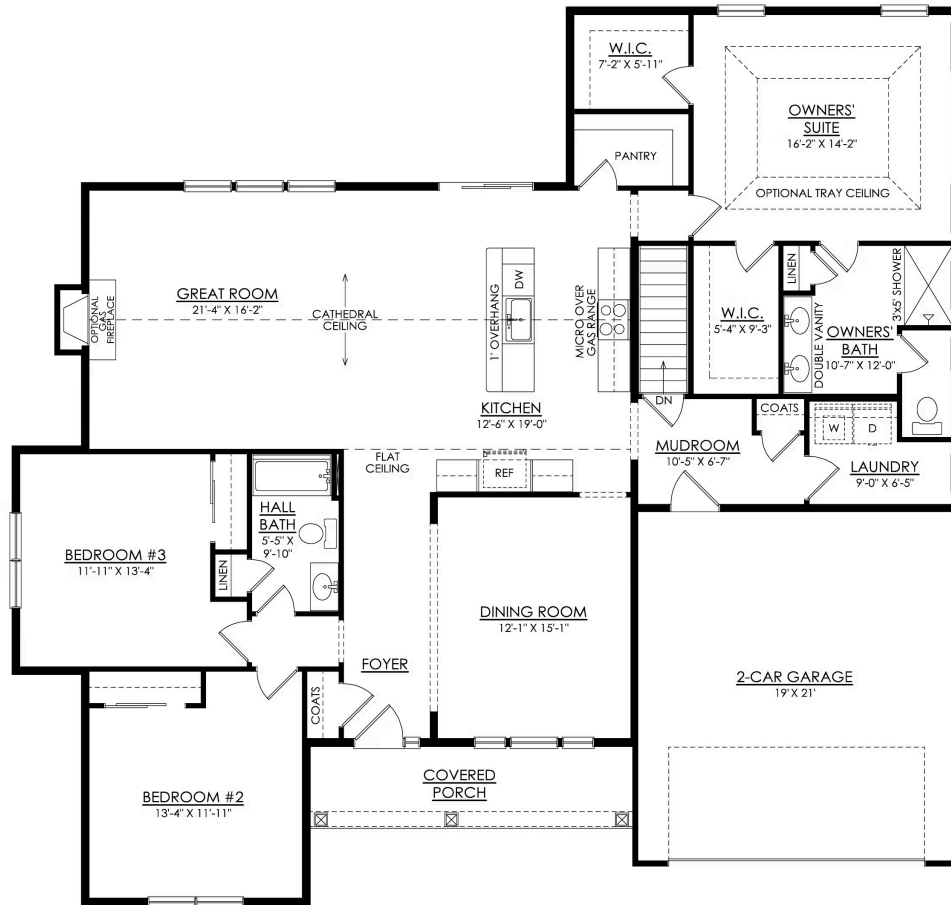
ROCKFORD COTTAGE 1ST FLOOR PLAN LIFESTYLE
