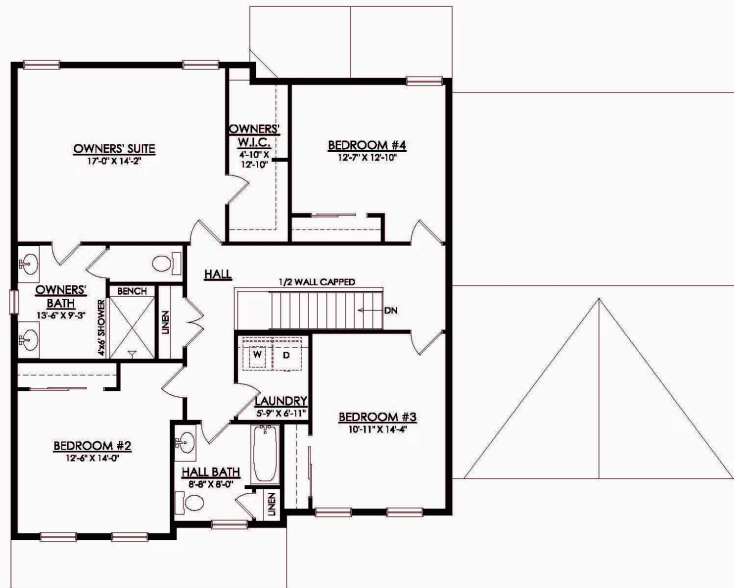
MAGNOLIA CRAFTSMAN 2ND FLOOR PLAN
