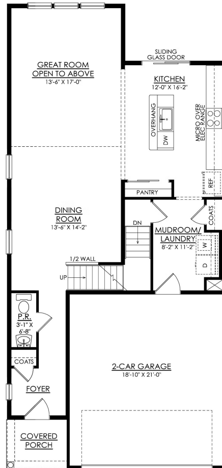
GRAYSON- 1ST FLOOR STARTING AT 2033 SF END UNIT
