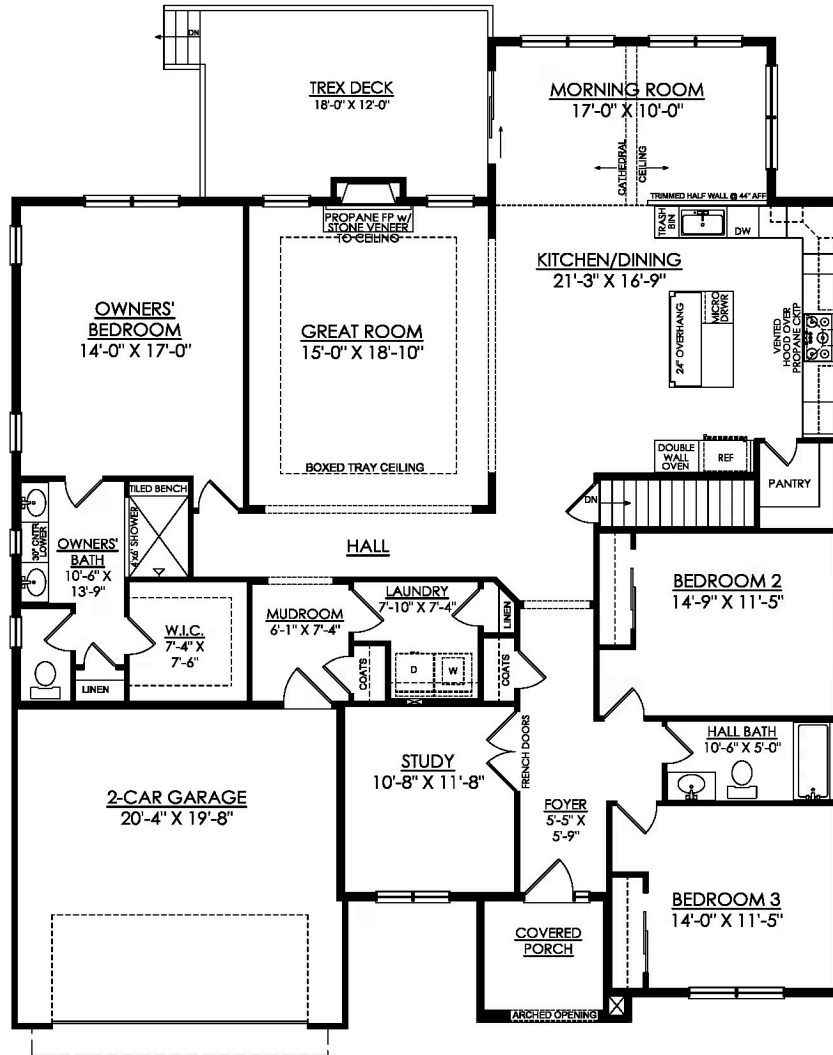
FOLINO COTTAGE 1ST FLOOR PLAN COVE AT MILLBROOK- CO-03
