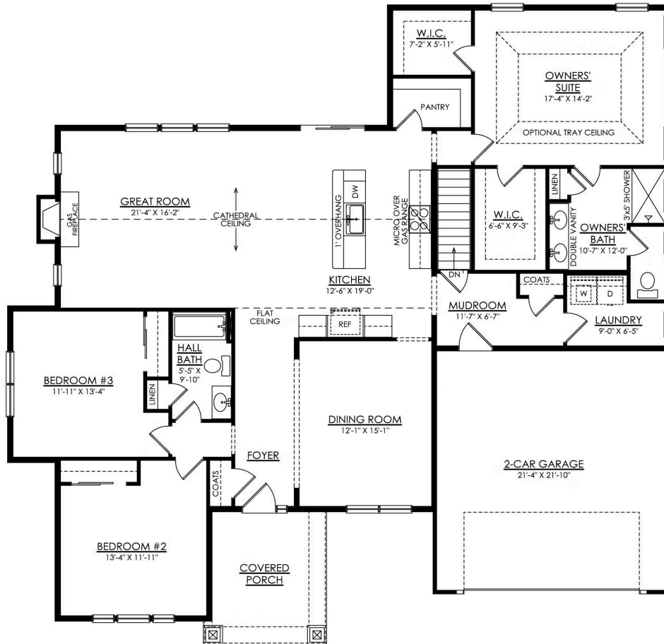
ROCKFORD CRAFTSMAN 1ST FLOOR PLAN PREMIER
