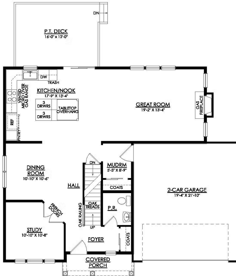
MADISON TRADITIONAL 1ST FLOOR PLAN HC09
