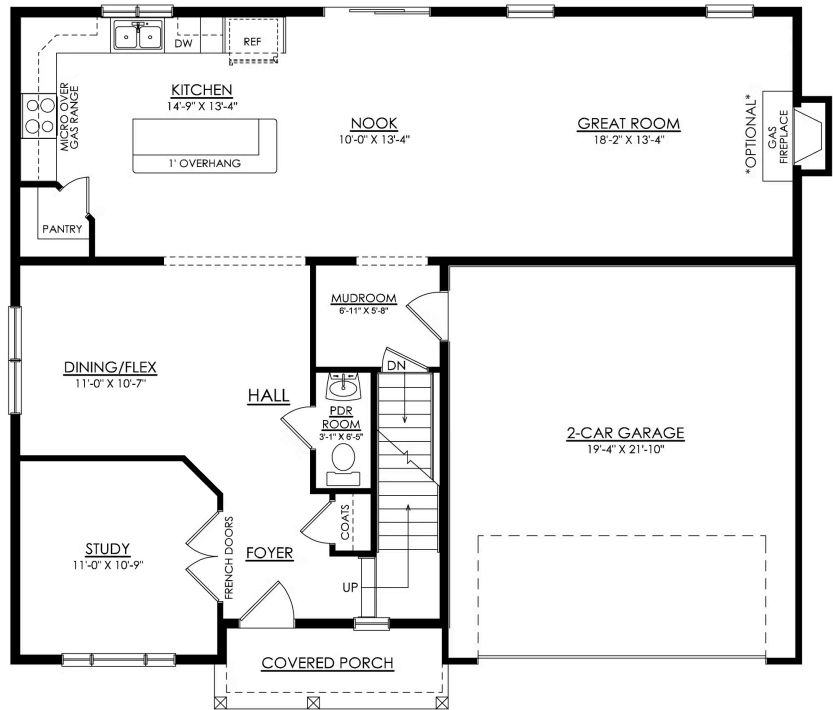
MORGAN TRADITIONAL STARTING AT 2648 SF 1ST FLOOR PLAN
