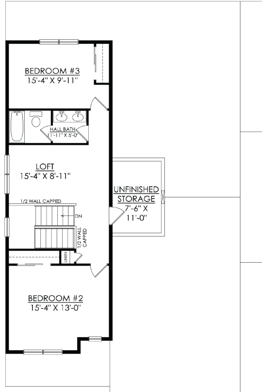
FRANKLYN TRADITIONAL 2ND FLOOR PLAN STARTING AT 2486 SF
