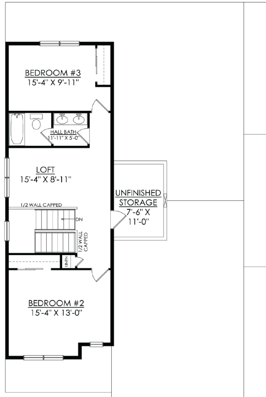
FRANKLYN CRAFTSMAN 2ND FLOOR PLAN STARTING AT 2486 SF
