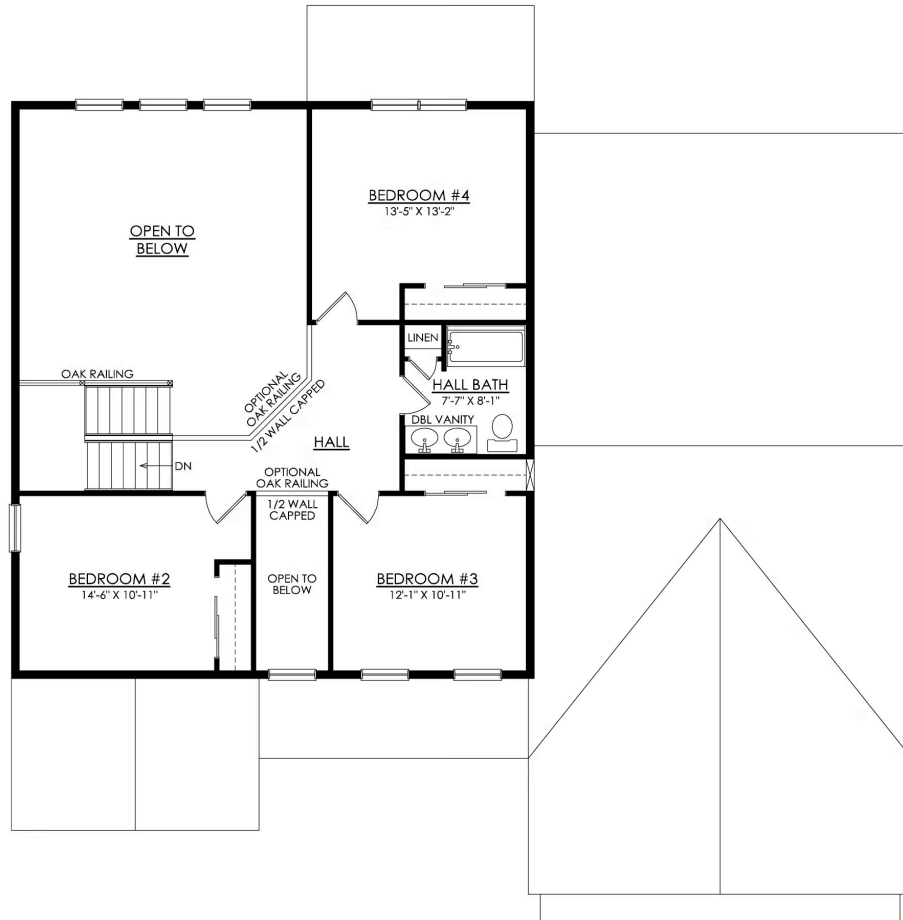
SIENNA FARMHOUSE 2ND FLOOR PLAN LIFE STYLE
