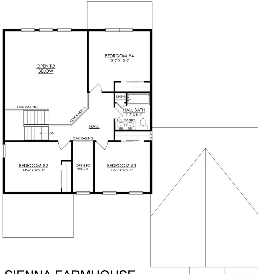
SIENNA FARMHOUSE 2ND FLOOR PLAN ESTATE
