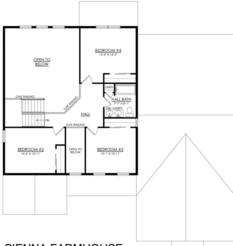
SIENNA FARMHOUSE 2ND FLOOR PLAN ESTATE
