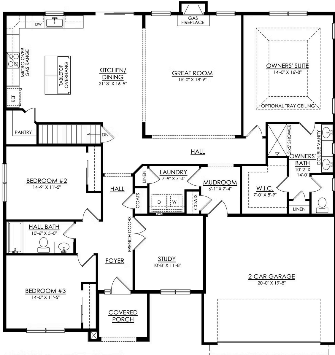
FOLINO COTTAGE 1ST FLOOR PLAN PREMIER
