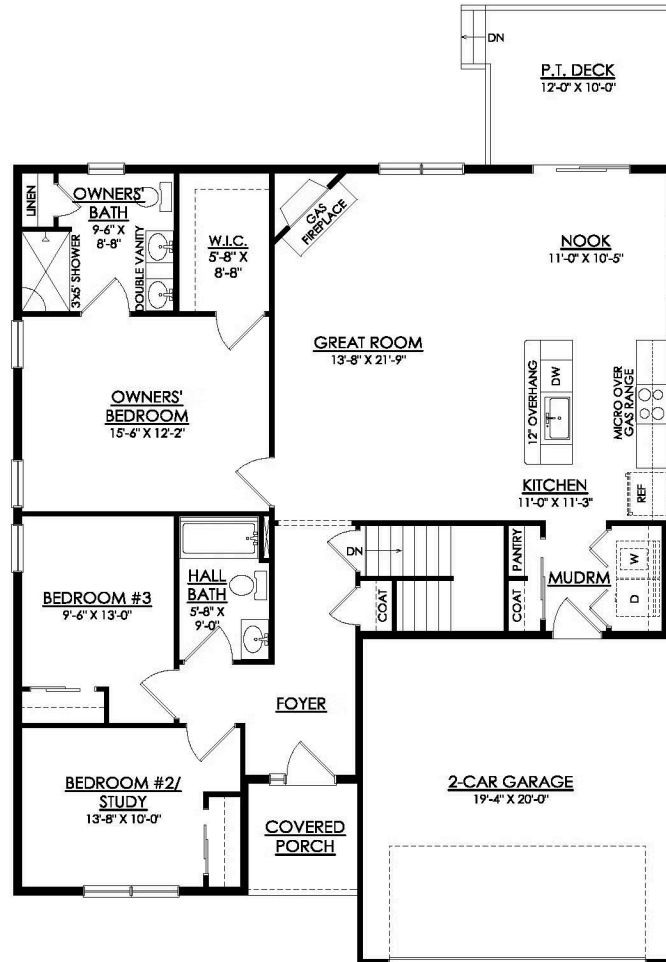
FIRST FLOOR PLAN G052- PINEHURST TRADITIONAL
