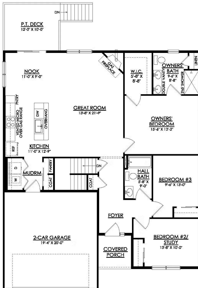
PINEHURST TRADITIONAL 1ST FLOOR PLAN GO87
