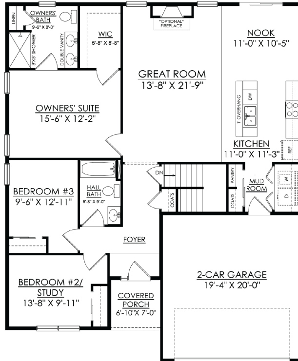
PINEHURST TRADITIONAL GOLDEN OAKS STARTING AT 1530 SF PLAN IS SHOWN WITH OPTIONAL FIREPLACE
