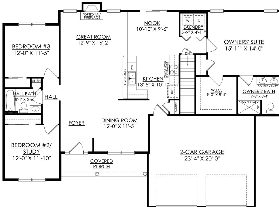
ST ANDREWS TRADITIONAL GOLDEN OAKS STARTING AT 1776 SF PLAN IS SHOWN WITH OPTIONAL FIREPLACE
